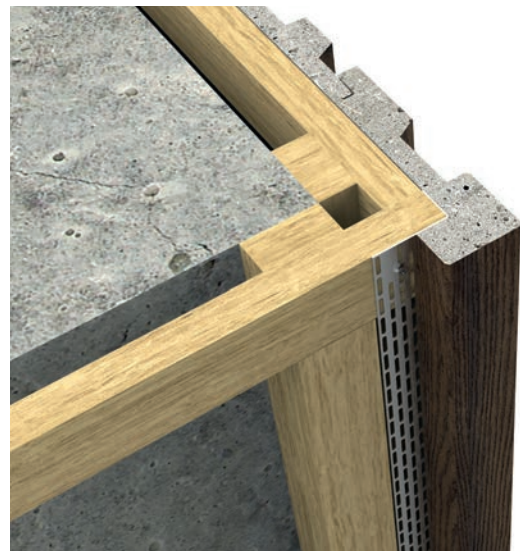
Fig. 8 - External corner detail
