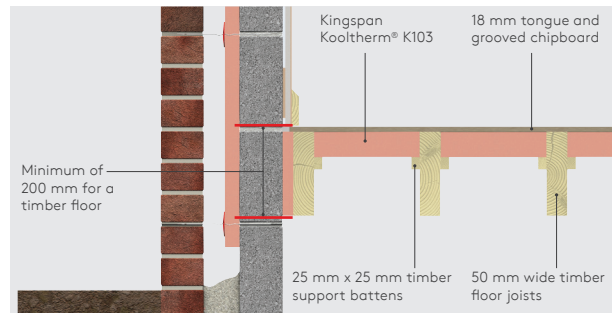
Figure 7: Complete timber floor insulation
